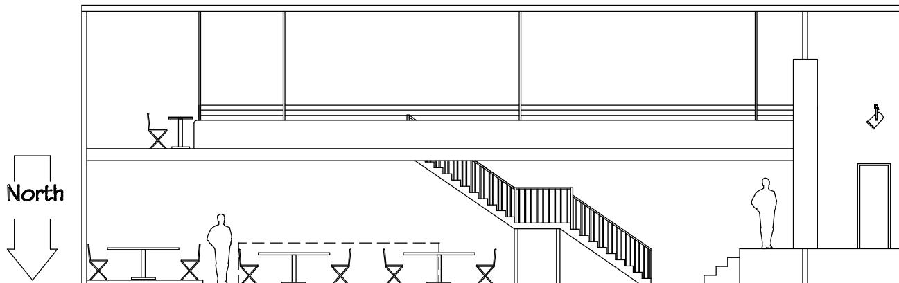
SECTION
